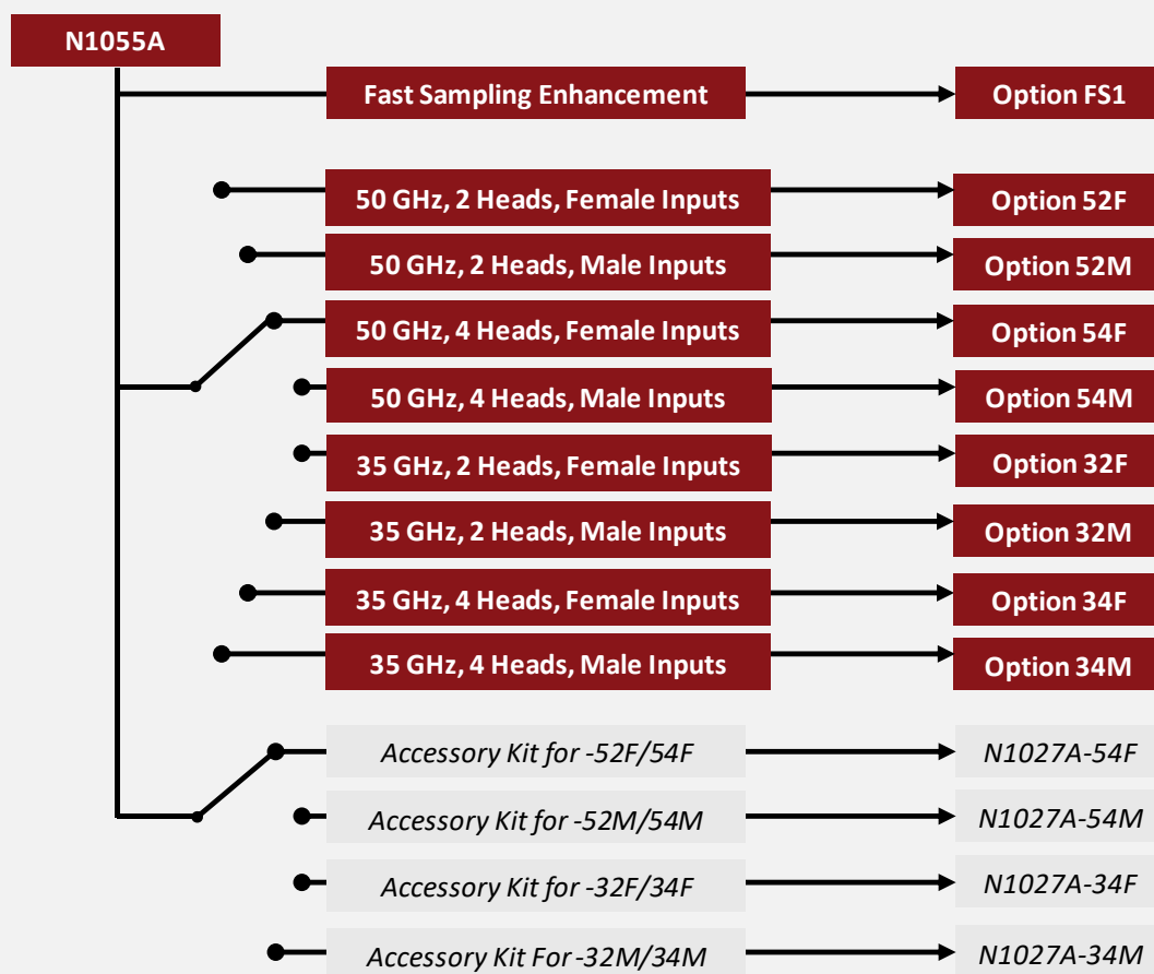
Figure 14. N1055A 50 GHz TDR/TDT modules with option 54M
