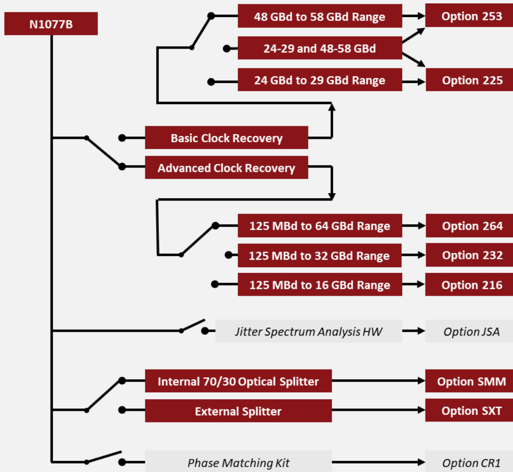
Figure 22. N1077B Multimode optical/electrical clock recovery with options 264 and SMM
