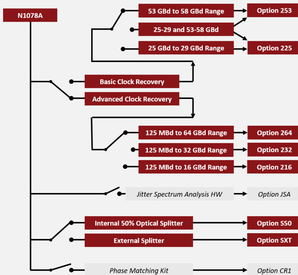
Figure 24. N1078A Single-mode optical/electrical clock recovery with options 264 and S50
