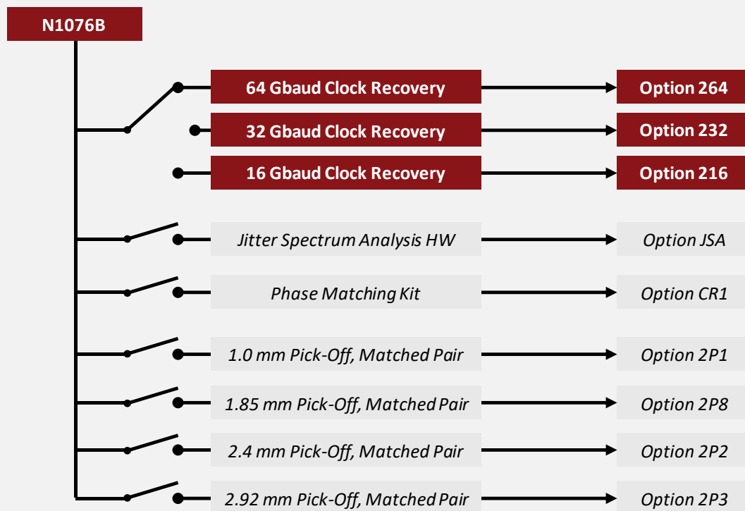
Figure 18. N1076B Electrical clock recovery with option 264
